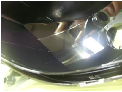
↑ None painting high glossy plastic injection
