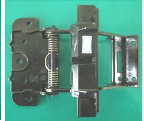
← RETAINER
